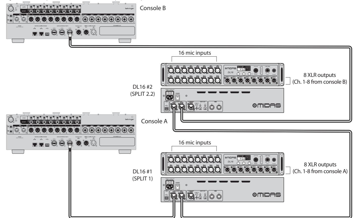
Fig. 5: Two-unit setup with two consoles and DL16s in Split 1.3 and Split 2.2 modes
