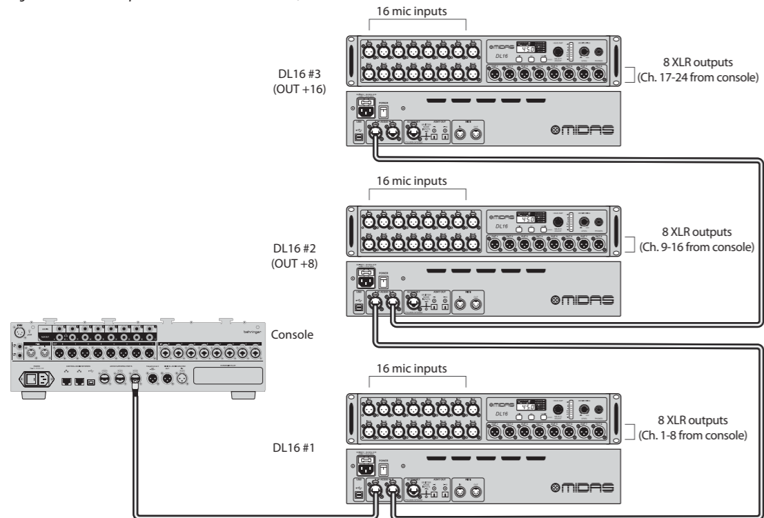
Fig. 2: Three-unit setup with DL16s in Standard mode, Standard +8 and Standard +16
