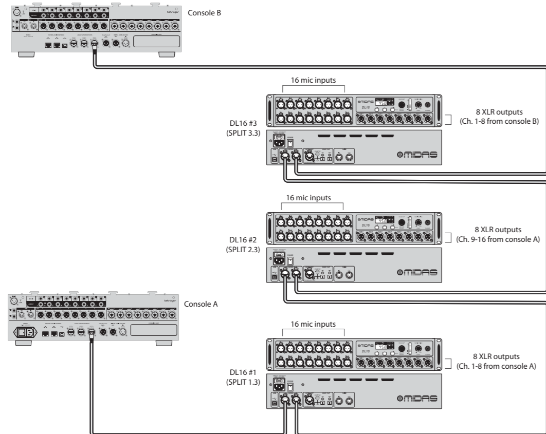
Fig. 4: Three-unit setup with two consoles and DL16s in Split 1.3, Split 2.3 and Split 3.3 modes
