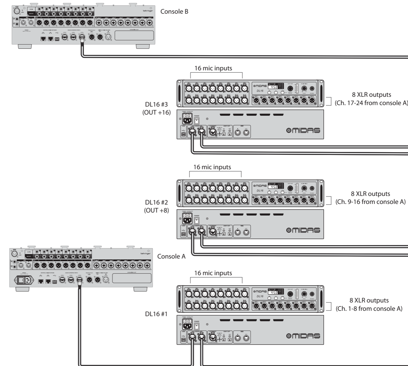
Fig. 3: Three-unit setup with two consoles and DL16s in Standard mode, Standard +8 and Standard +16
