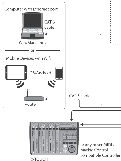
ETHERNET mode
